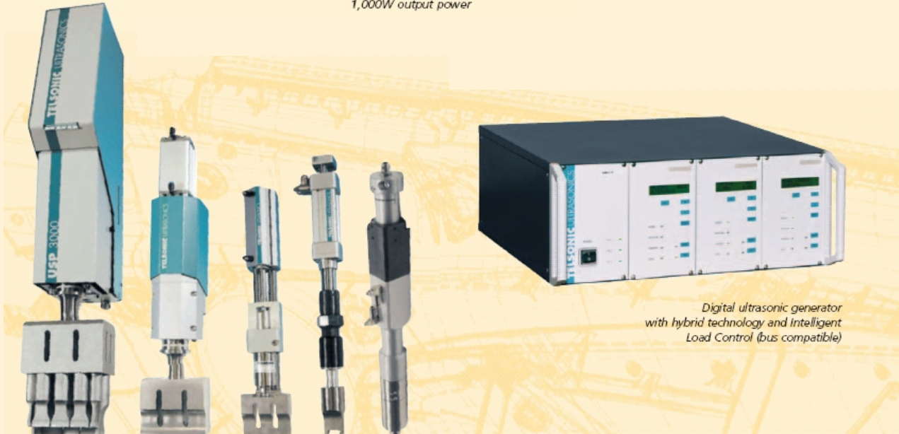
Various ultrasonic actuators with up to 3,000N force
