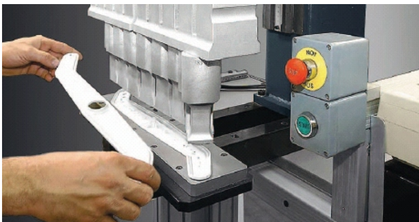
Welding of dishwasher spray arm utilising twin mother/daughter sonotrode.
