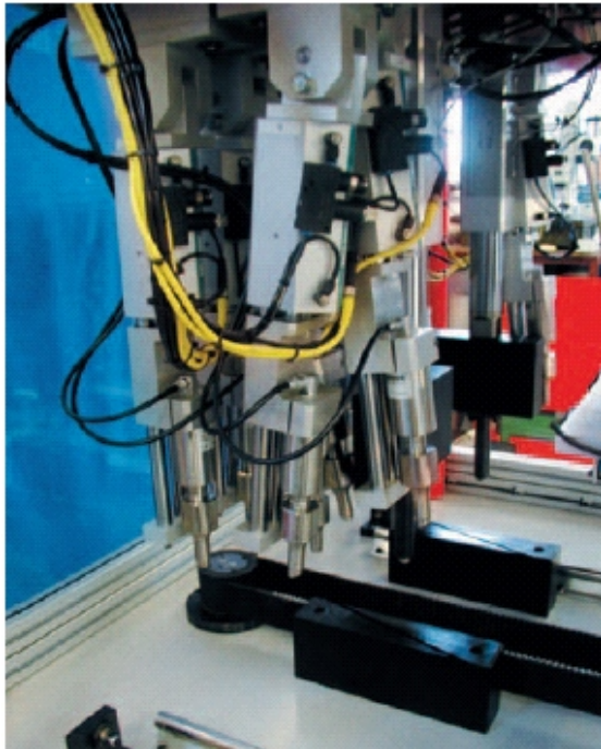
Multi-headed welding system for the welding of acoustic material to polypropylene moulding.
