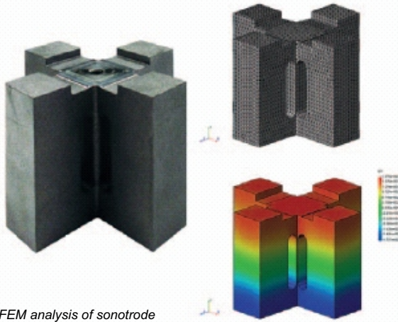
FEM analysis of sonotrode
