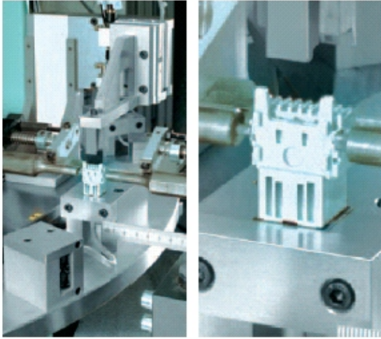
Rotary table with integrated precision actuators
